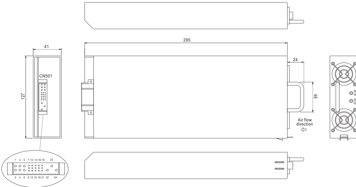
Input / Output Connector Pin No. Assignment(CN501) : Postronic PCB24W9M400A1
