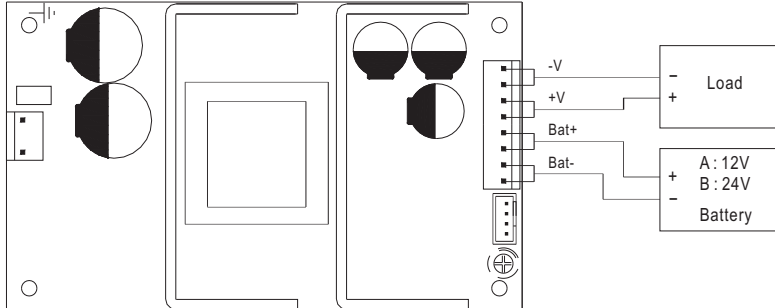
Fig 1.1 Suggested system connection
