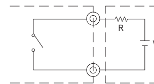
Fig 2.2 Internal circuit of AC OK (Battery Low)
