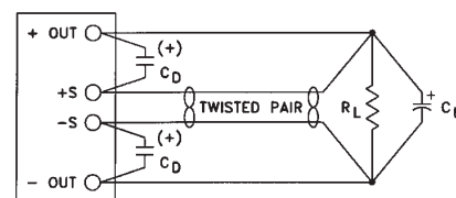
Figure 1 - Output sense connections
